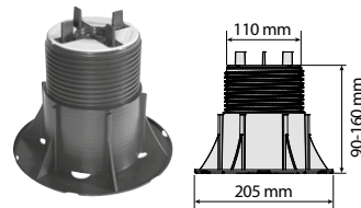
201009 Supporto regolabile Adjustable paving support mm 90/160
